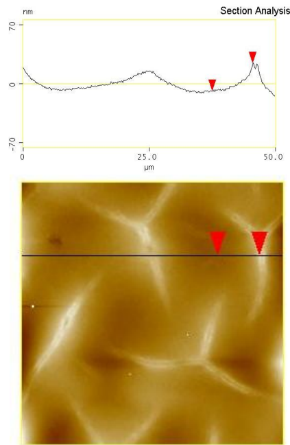
Figure 3.11: AFM image and amplitude measurement of 800 nm thick film with pattern 1. The section analysis of an amplitude measurement of a wrinkle is above.
